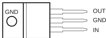
KCS (TO-220) PACKAGE (TOP VIEW)
